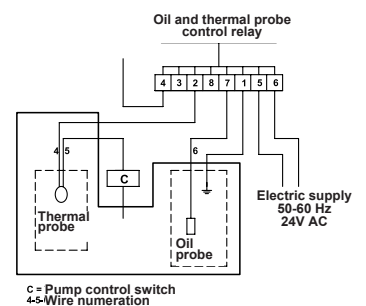
Fig. 13 Thermal probe connection
